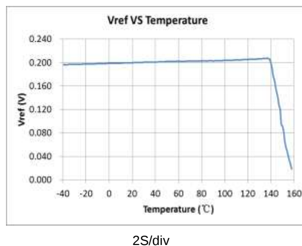
Thermal regulation curve
