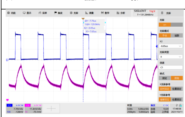
图7: 5Vin/6LEDs (CH1:V DRAIN CH4:I OUT )
