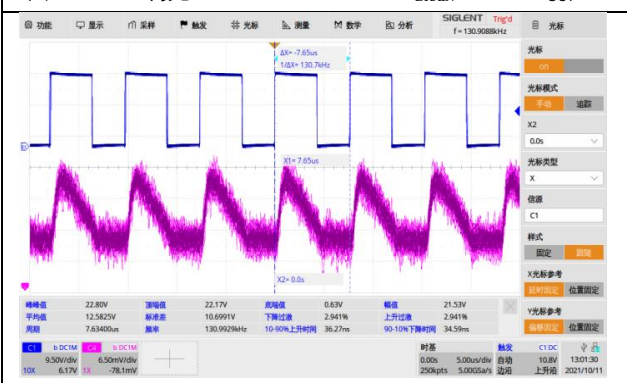
图3: PWM调光 (4KHZ/10%) (CH2:V DRAIN CH3:I OUT )
