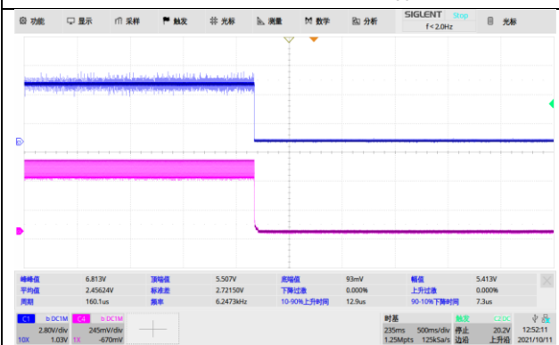
图1: PWM至低电平 (CH1:V DIM CH4:I OUT )
