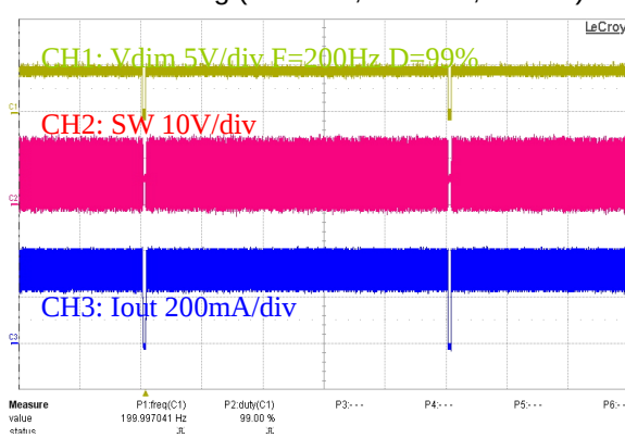
PWM dimming (Vin=12V, L=47uH, 3xLED)
