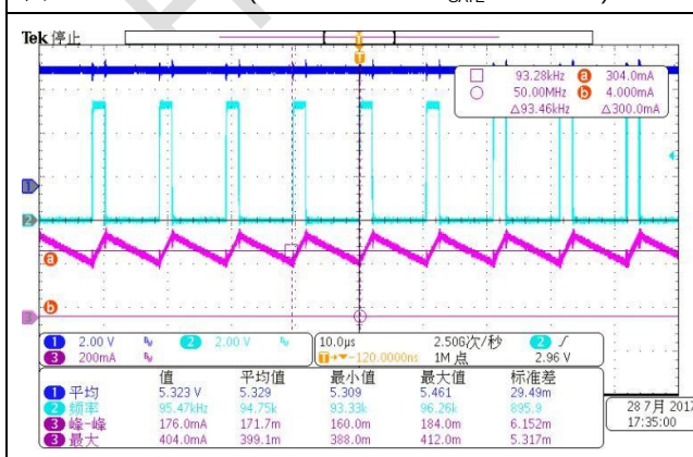
图1: 48Vin/3LEDs (CH1:VDD CH2:V GATE CH3:I OUT )
