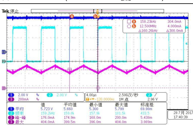
图2: 48Vin/8LEDs (CH1:VDD CH2:V GATE CH3:I OUT )
