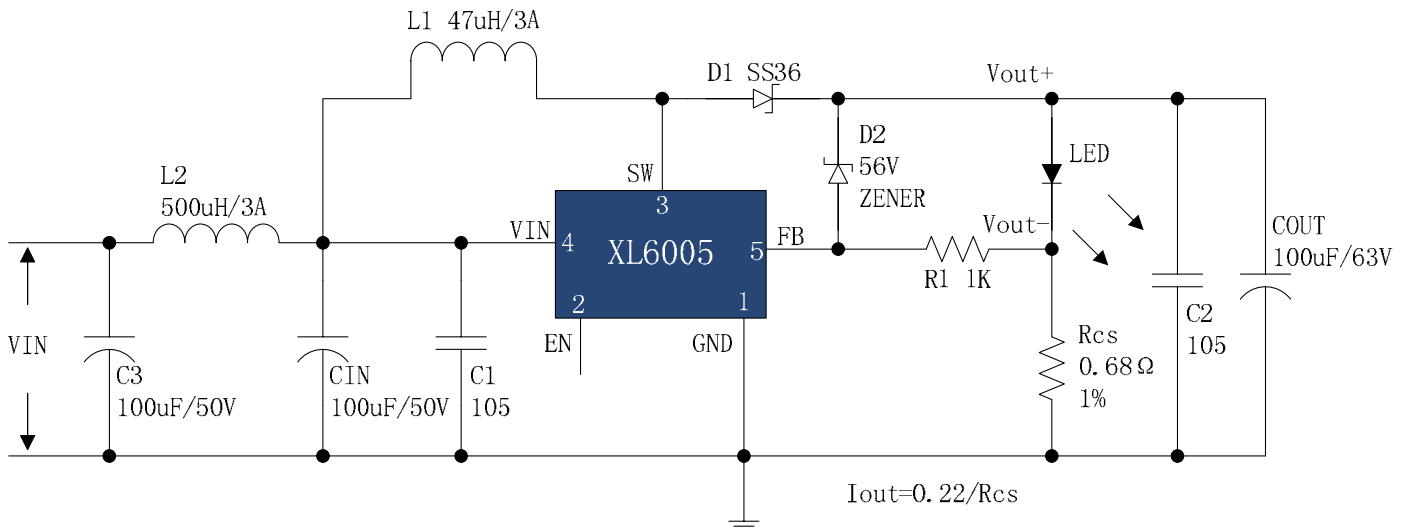
XL6005 VIN=DC5V~DC32V, IOUT=320mA Typical Application Circuit
